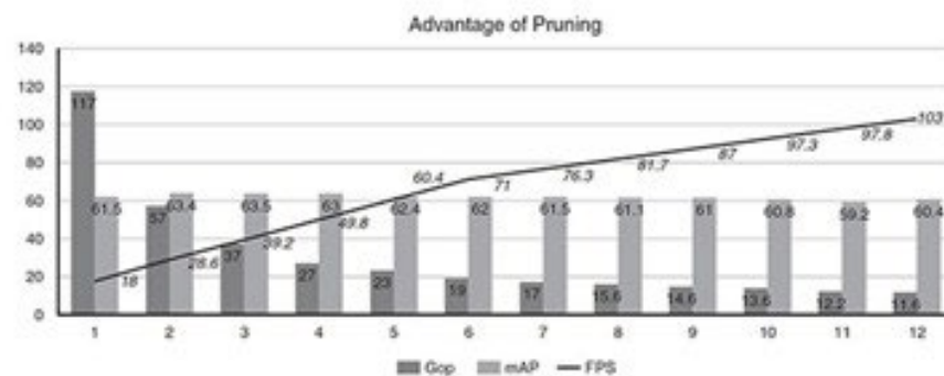
Figure 3: After a relatively few iterations, pruning can reduce model complexity (Gop) by 10X and improve performance (FPS) by 5X, with only a 1% reduction in accuracy (mAP). Image source: AMD Xilinx
