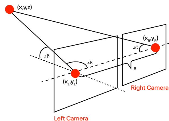
Figure 4: A standard stereo vision system example.
